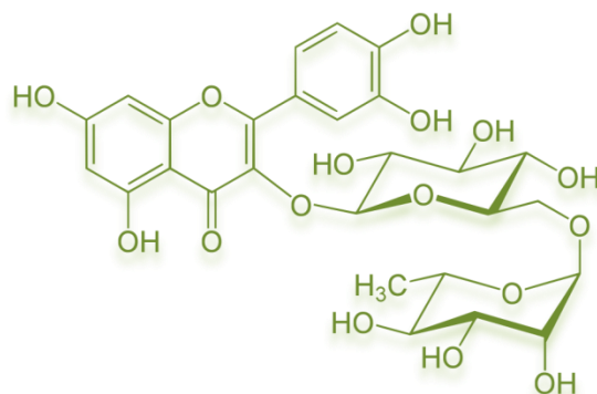
Quercetin-3-O-rutinoside
